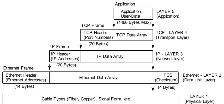
Figure 1: CONSTRUCTION OF A TCP/IP-ETHERNET DATA PACKET
